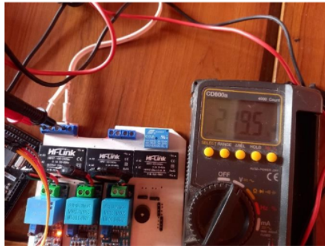
Gambar 9 Tegangan Phase R
