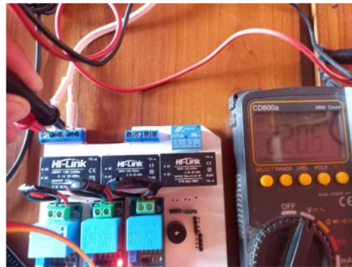
Gambar 12 Tegangan Phase S
