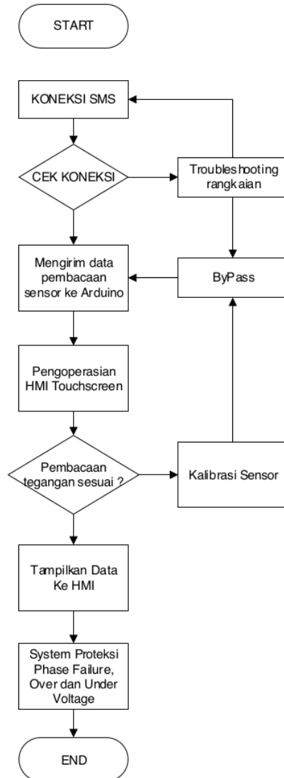
Gambar 2. Flowchart
