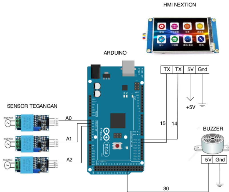
Gambar 3. Diagram Wiring
