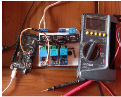
Gambar 8 Proses testing tegangan 220VAC
