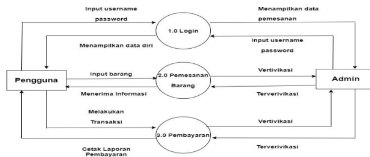
Gambar 4. DFD Level 1
