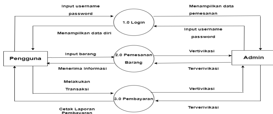
Gambar 4. DFD Level 1
