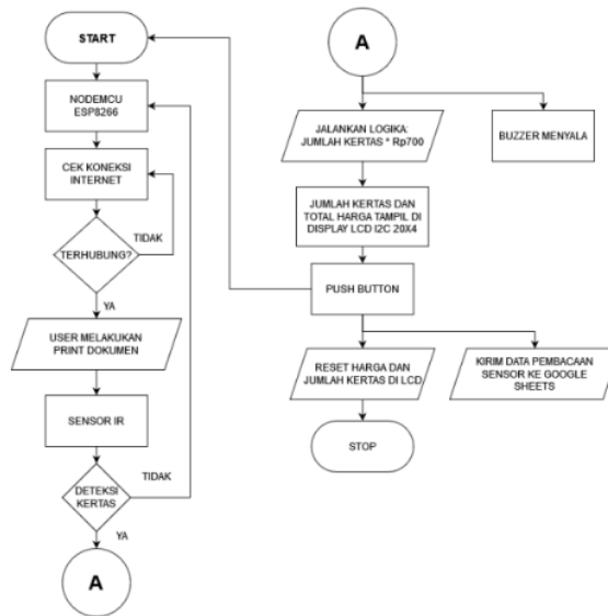
Gambar 1. Flowchart Sistem
