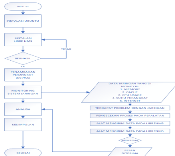
Gambar 2. Flowchart penelitian [1]
