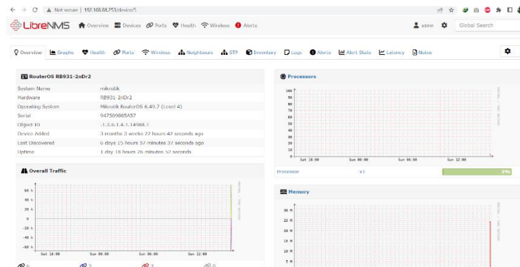
Gambar 7. Dashboard alat
