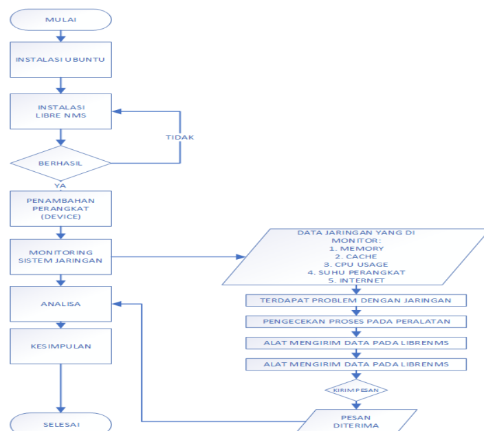
Gambar 2. Flowchart penelitian [1]
