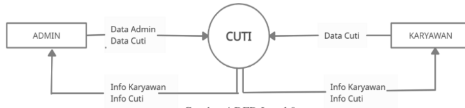
Gambar 4 DFD Level 0
