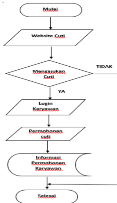
Gambar 2. Flowchart User
