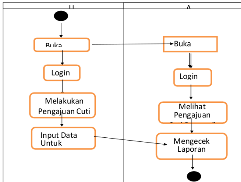
Gambar 3 .Activity Daigram
