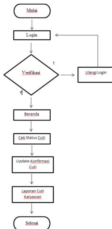
Gambar 1 Flowchart Admin.
