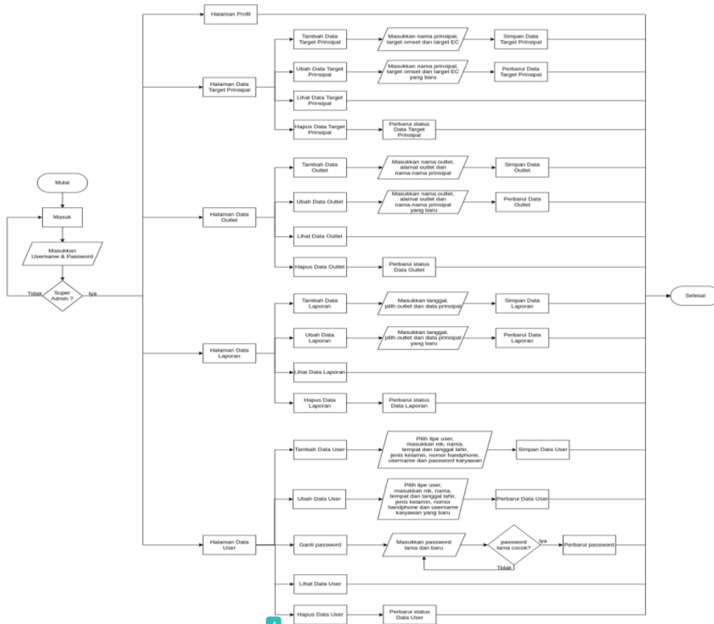
Gambar 3. Flowchart Admin
