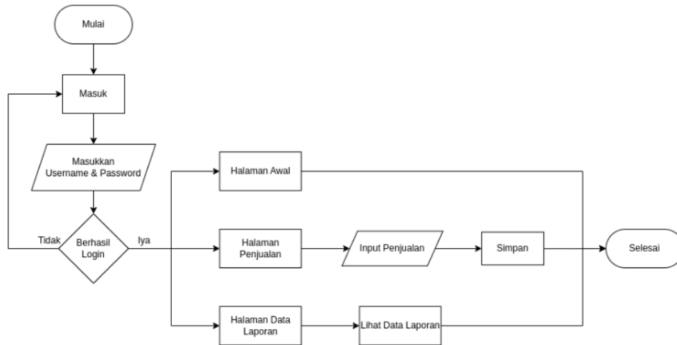
Gambar 4. Flowchart Sales
