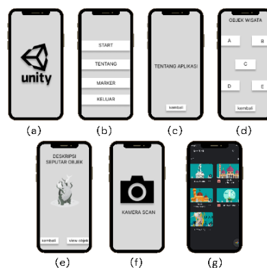
Gambar 4. Desain User Interface
