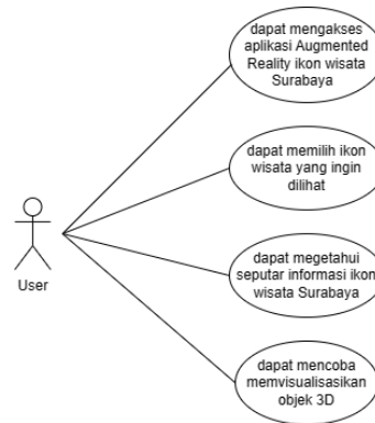
Gambar 3. Use Case Diagram
