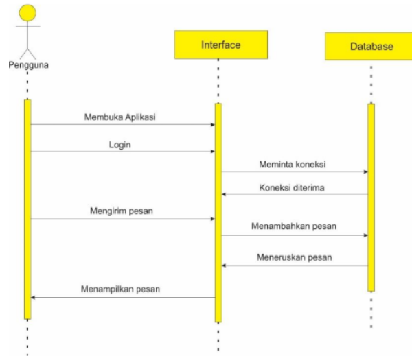
Gambar 2. Sequence Diagram
