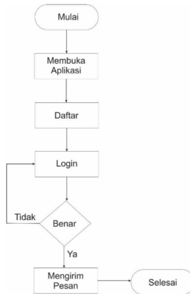
Gambar 3. Flowchart Diagram
