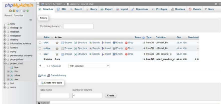
Gambar 6. Database
