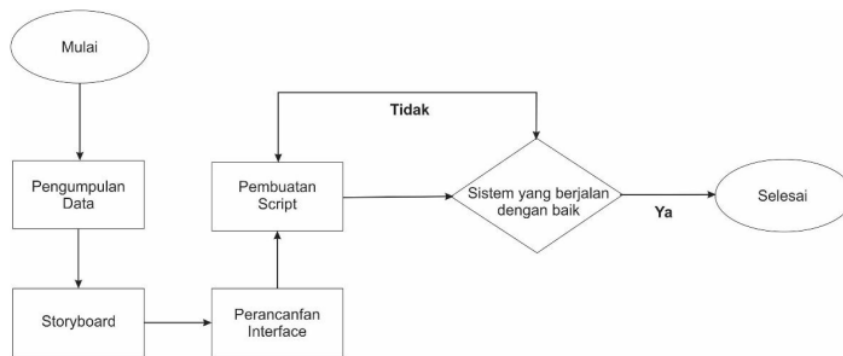
Gambar 5. Storyboard
