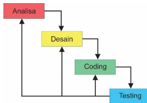
Gambar 1. Model Waterfall
