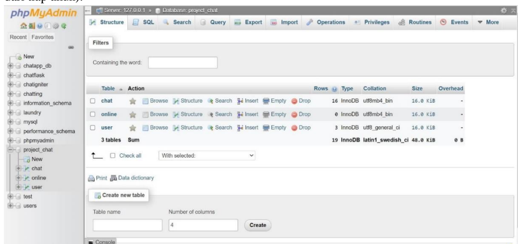
Gambar 6. Database
