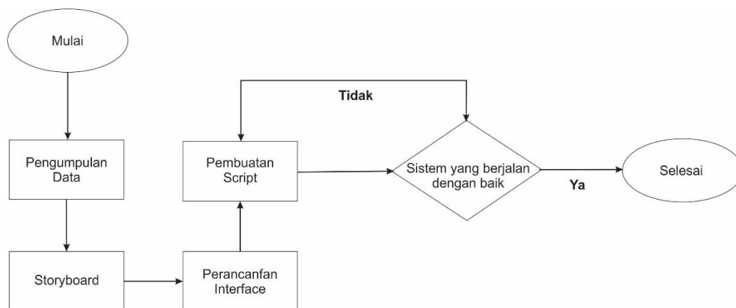
Gambar 5. Storyboard
