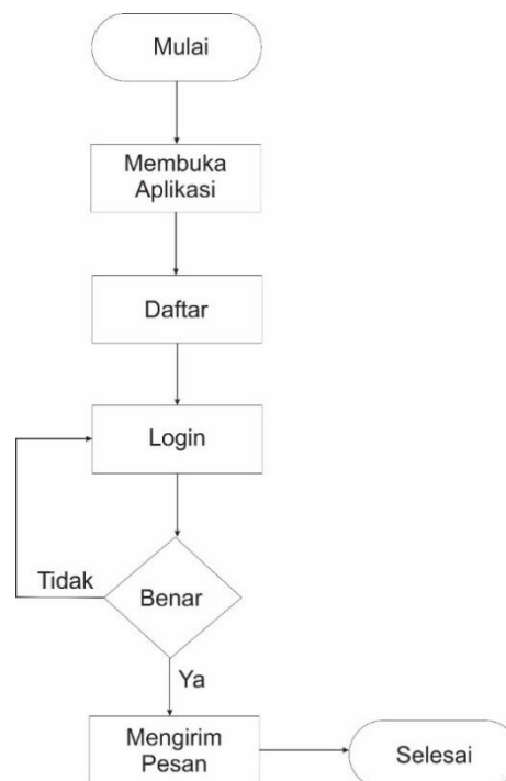
Gambar 4. Flowchart Diagram
