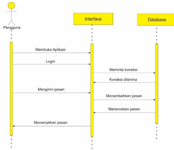
Gambar 3. Sequence Diagram
