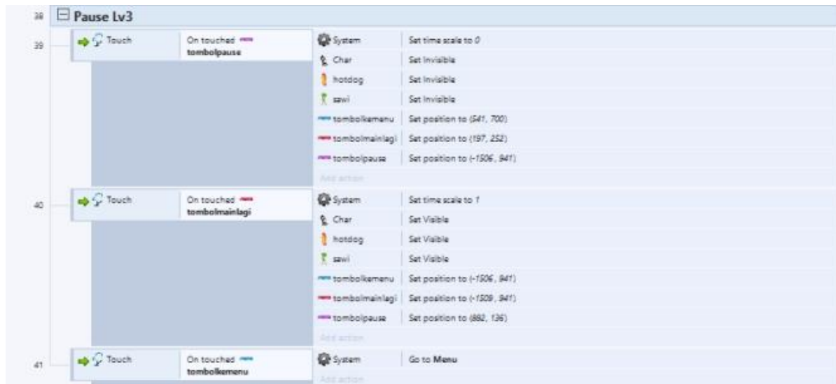
Gambar 20. Source Code Tampilan Pause
