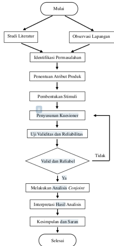
Gambar 2. Flowchart Penelitian
