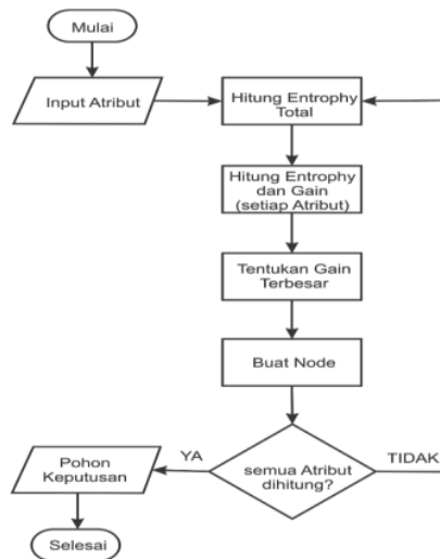
Gambar 2. Flowchart
