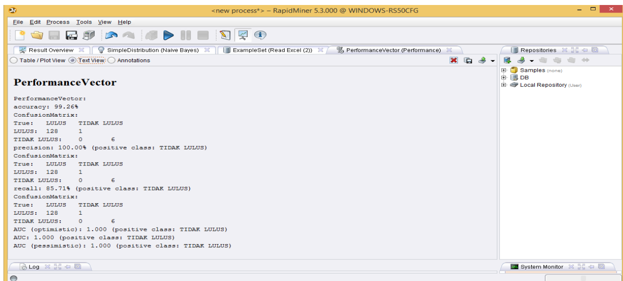
Gambar 13. Performance vector
