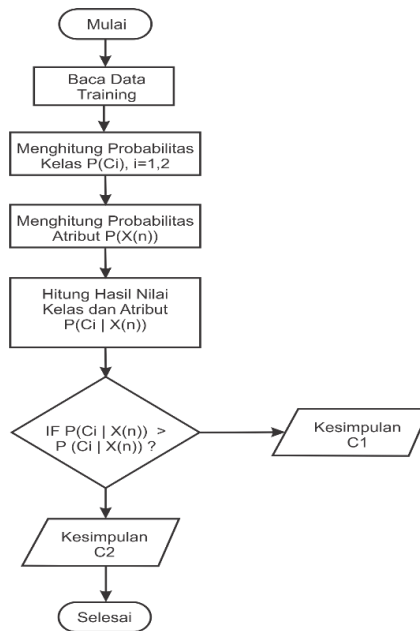
Gambar 2. Flowchart naïve bayes
