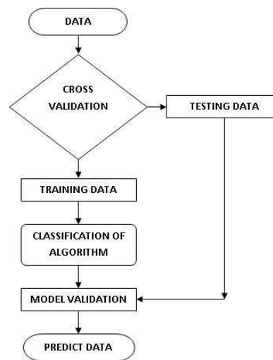
Gambar 8. Flowchart rapidminer
