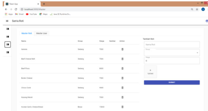
Gambar 12. Master Roti
