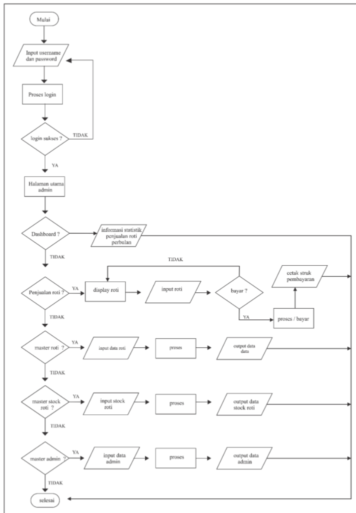
Gambar 2. Flowchart Sistem
