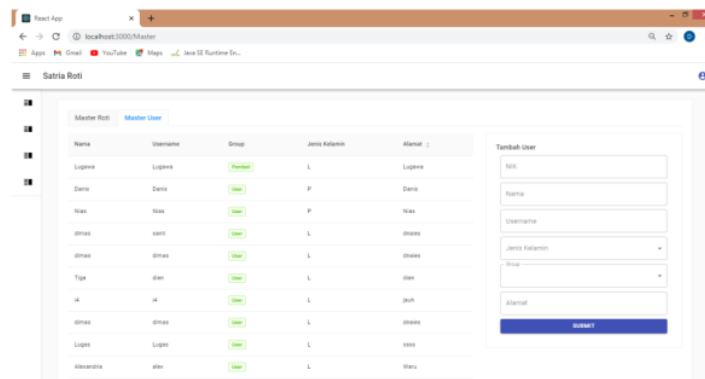
Gambar 13. Master Admin
