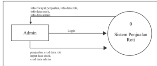
Gambar 3. DFD LEVEL 0
