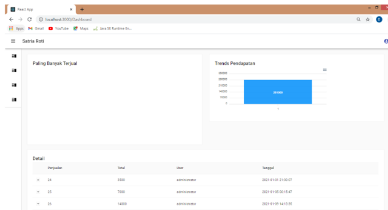
Gambar 8. Halaman Dashboard
