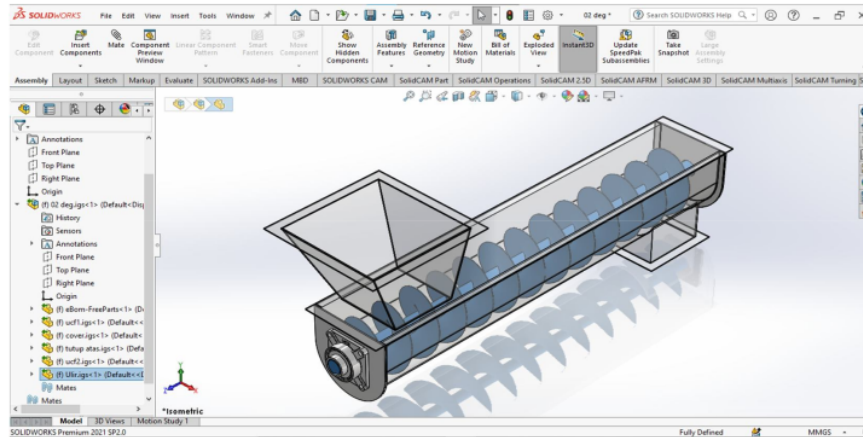
Figure 1. 3D Model of Screw Conveyor
