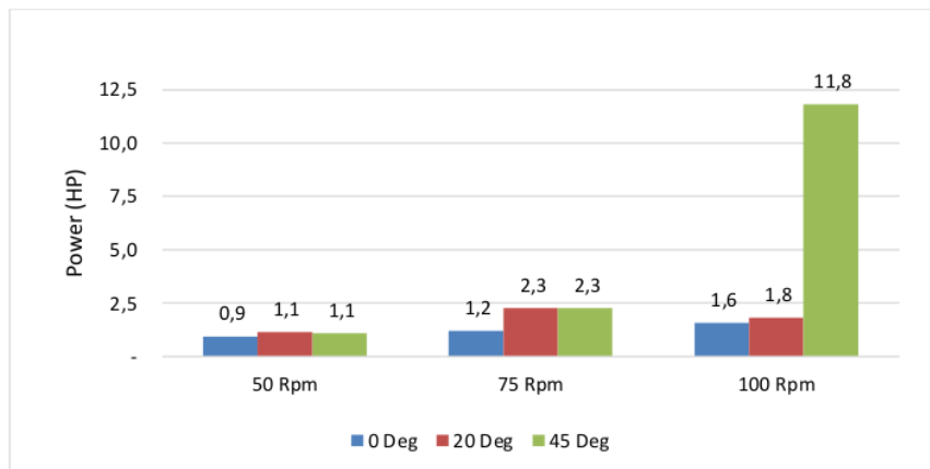
Graphic 4. DEM Simulation results for horsepower
