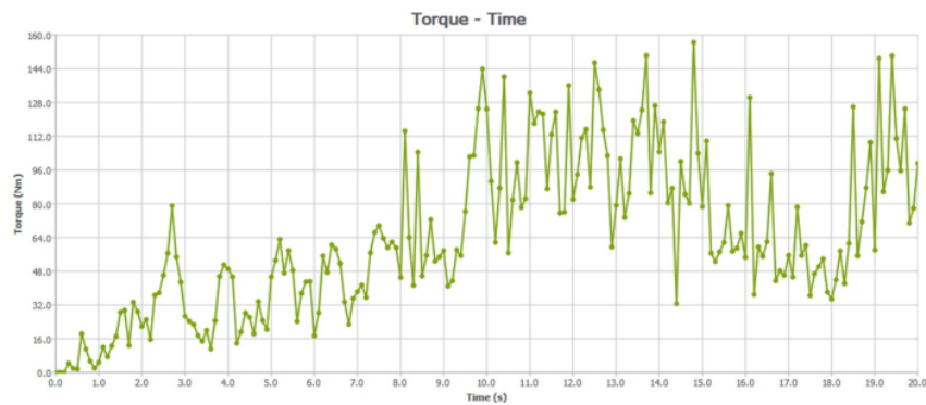
Graphic 2. Torque simulation results of 45 degrees on 50 Rpm
