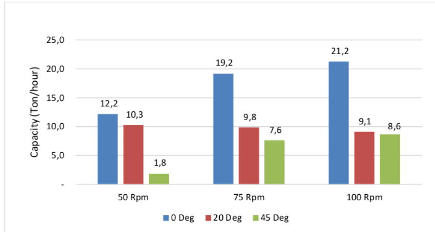
Graphic 3. DEM Simulation results for capacity
