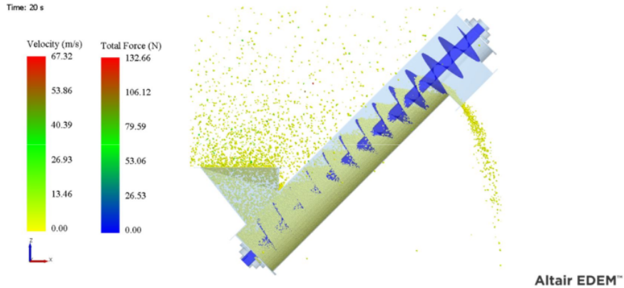
Figure 3. Simulation on 45 Degree modeling with 50 Rpm
