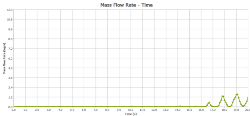
Graphic 1. Mass flow simulation results of 45 degrees on 50 Rpm
