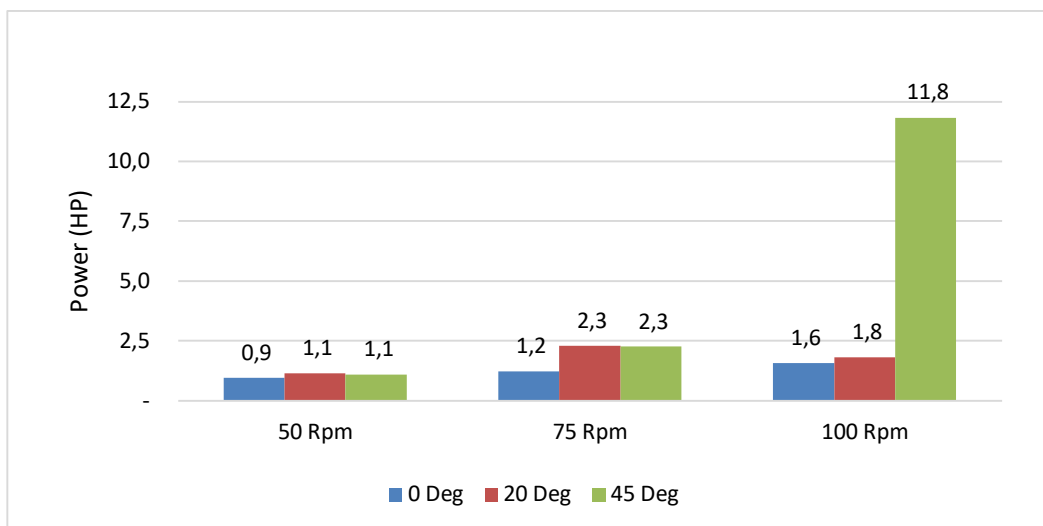
Graphic 4. DEM Simulation results for horsepower
