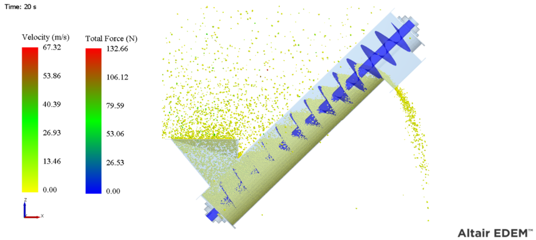
Figure 3. Simulation on 45 Degree modeling with 50 Rpm
