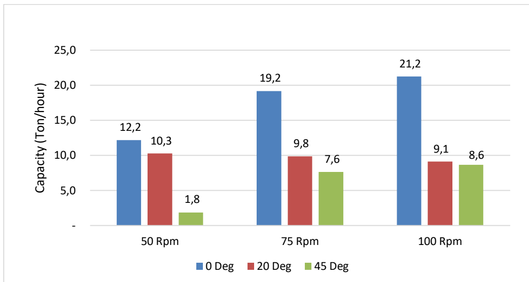
Graphic 3. DEM Simulation results for capacity
