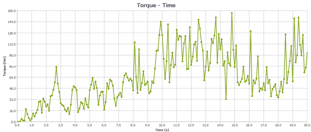
Graphic 2. Torque simulation results of 45 degrees on 50 Rpm
