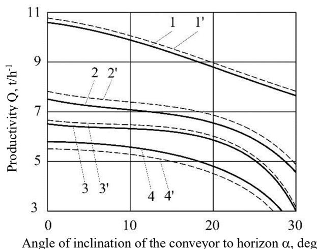
Graphic 5. Productivity Q of the conveyor with a screw working body (solid line) and bladed one (dashed line) at 300 rpm (1 – sand; 2 – peas; 3 – wheat; 4 – corn).
