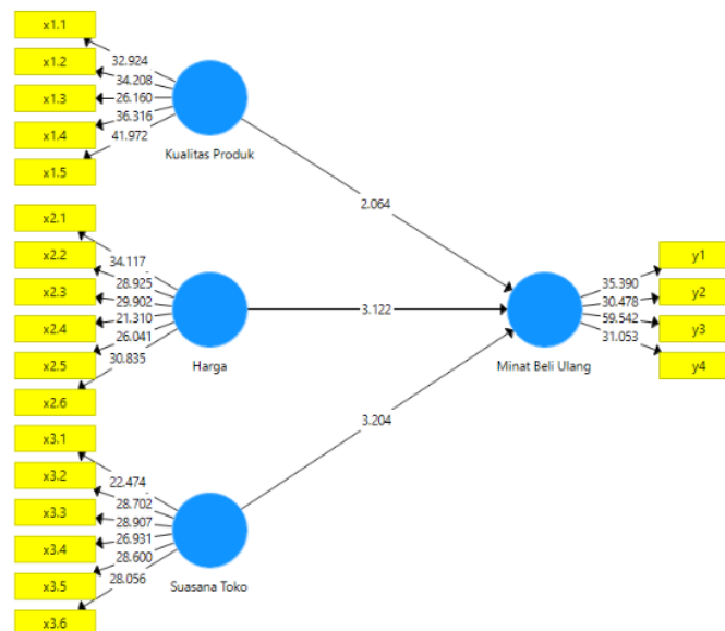
Gambar 1. Bootstrapping Test Results
