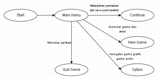
Gambar 2. Finite state machine Main Menu
