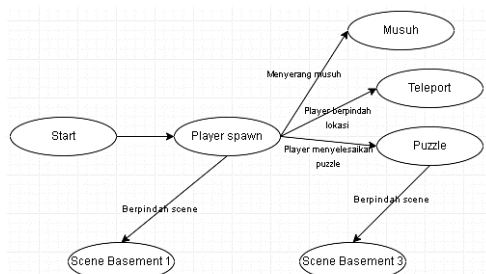
Gambar 4. Finite state machine Basement 2
