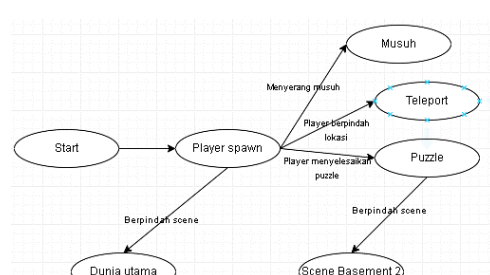
Gambar 3. Finite state machine Basement 1
