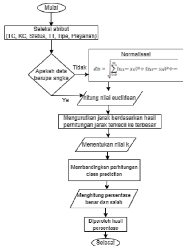
Gambar 1. Flowchart Proses K-NN
