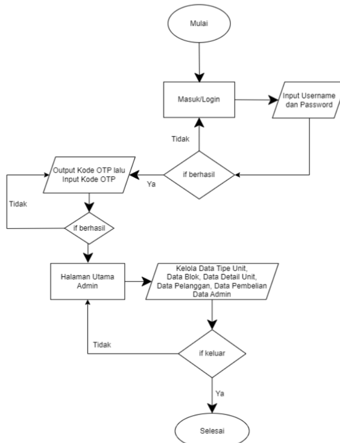
Gambar 1. Flowchart Admin
