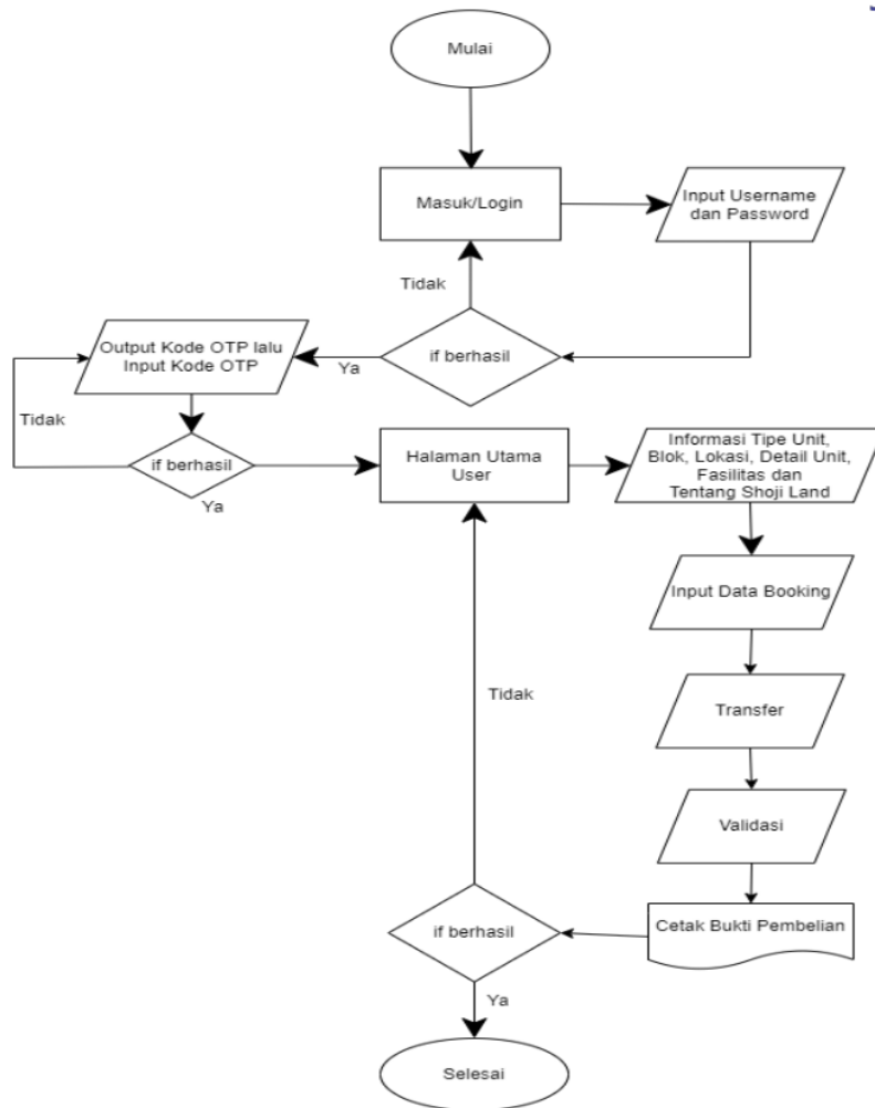
Gambar 2. Flowchart User
