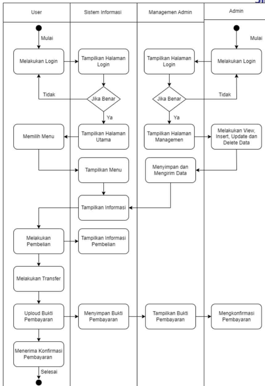
Gambar 3. Activity Diagram
