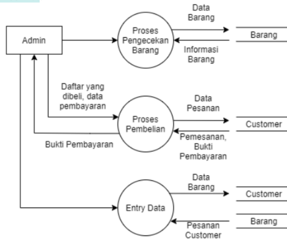
Gambar 5. DFD Level 1
