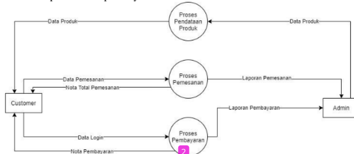
Gambar 4. DFD Level 0
