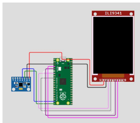
Gambar 1. Wiring Diagram
