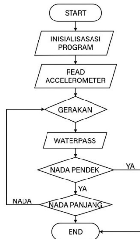
Gambar 2. Flow Chart
