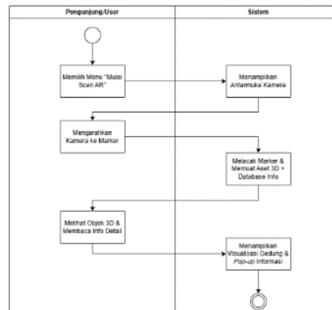
Gambar 4. Activity Diagram Pemindaian Penanda
