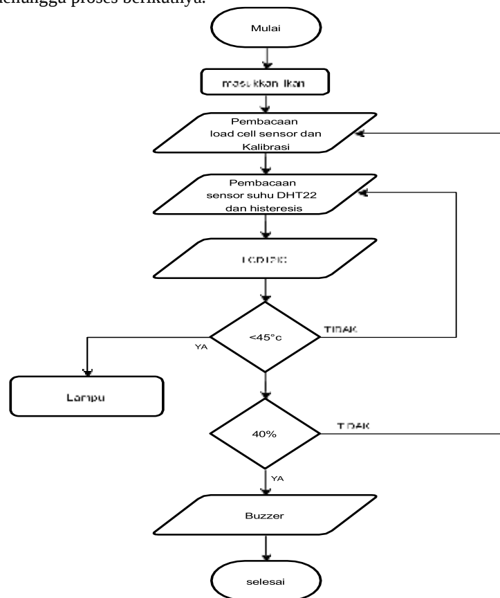
Gambar 2. Flowchart System
