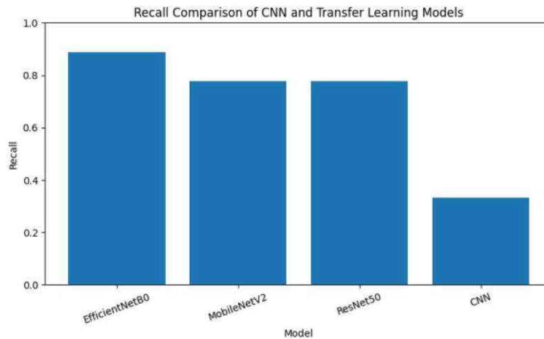
Figure 10. Recall Comparison of CNN and Transfer Learning Models
