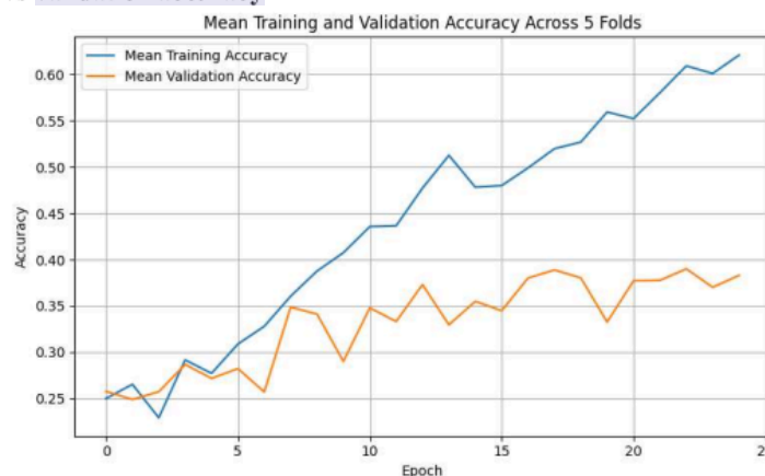
Figure 6. Mean Training and Validation Accuracy Across 5 Folds
