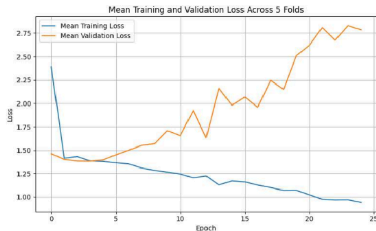
Figure 7. Mean Training and Validation Loss Across 5 Folds
