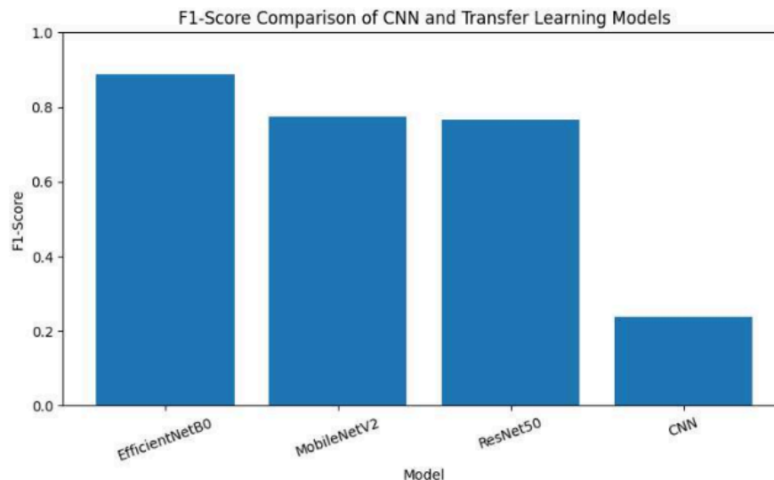
Figure 11. F1-Score Comparison of CNN and Transfer Learning Models
