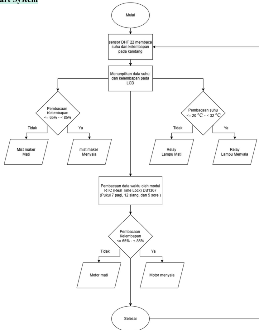
Gambar 3. Flowchart System
