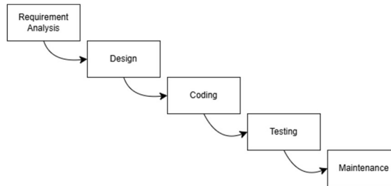
Gambar 2.1 Metode Waterfall
