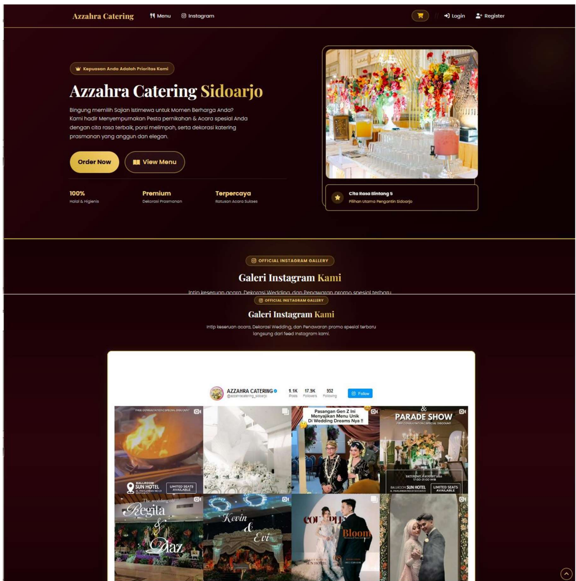
Gambar 3.1 Beranda Website
