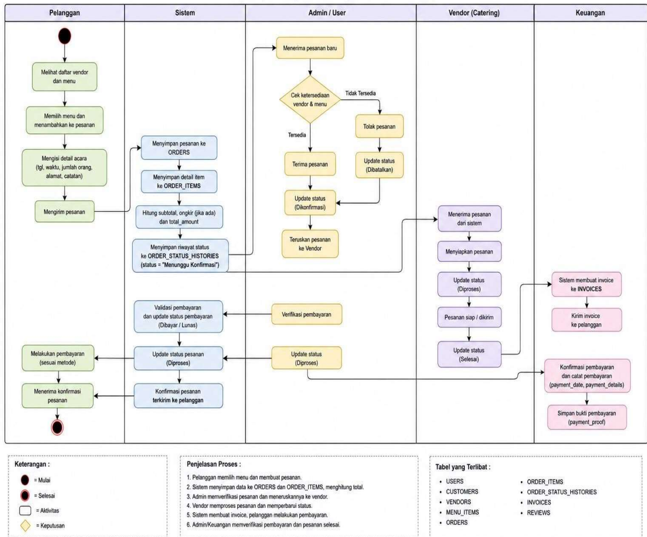
Gambar 2.3 Activity Diagram
