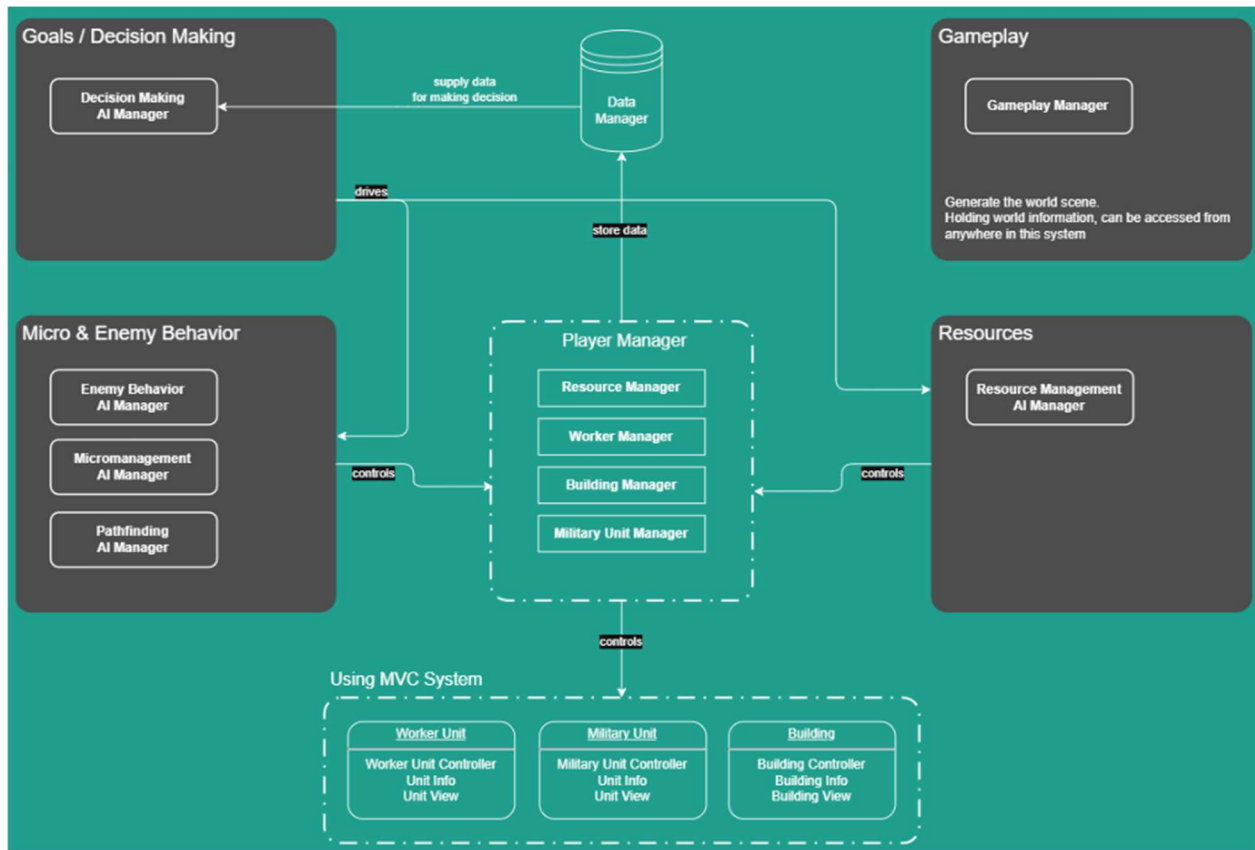
Gambar 1. Diagram Sistem Enemy AI
