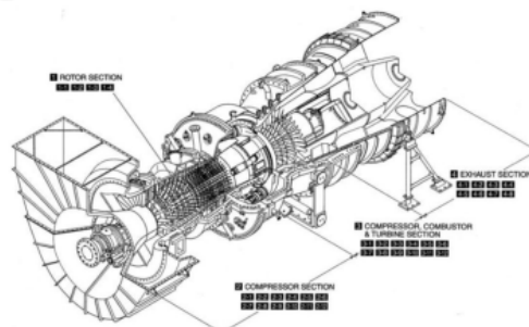
Gambar 3. Gas turbin M701D (Sumber: PT. XYZ)
