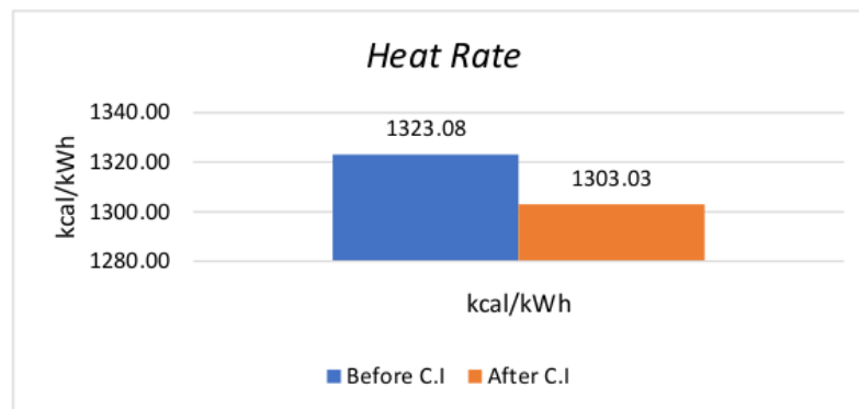
Gambar 11. Heat Rate
