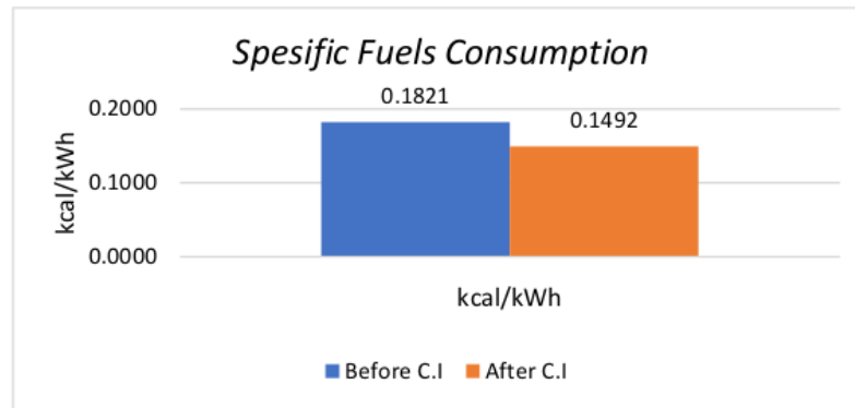
Gambar 12. Grafik Specific Fuels Consumption
