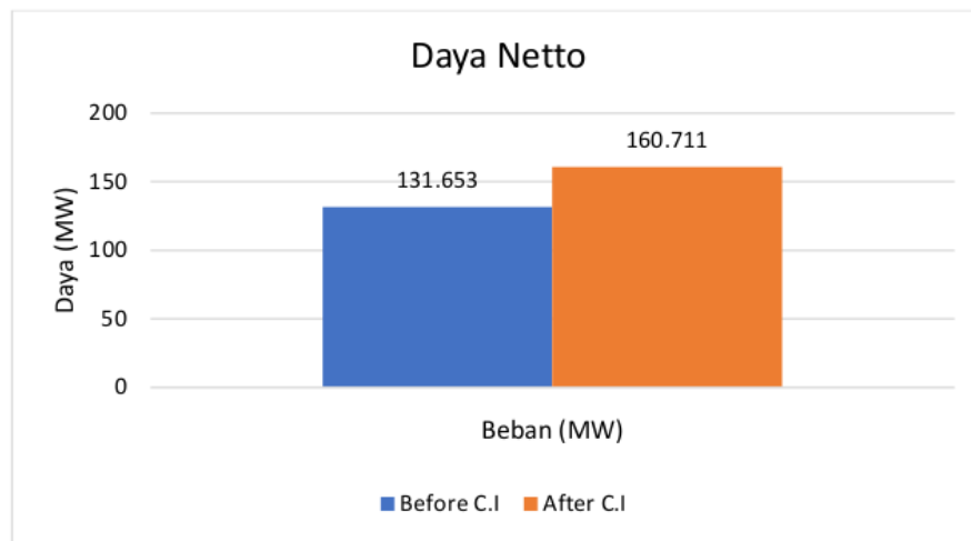
Gambar 7. Daya Netto
