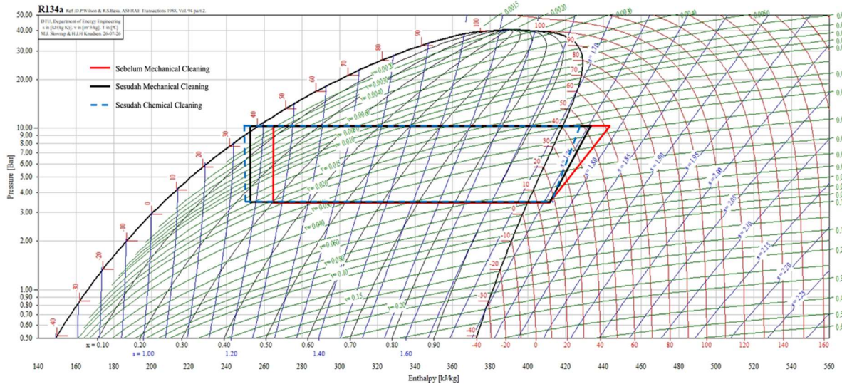
Gambar 7. Komparasi Diagram P-h Refrigeran R134a Load 55%
