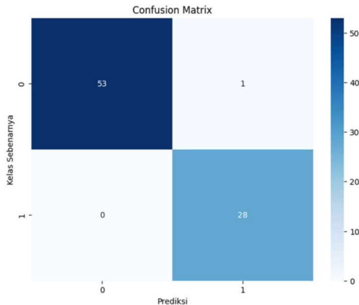
Gambar 3 Confusion Matrix
