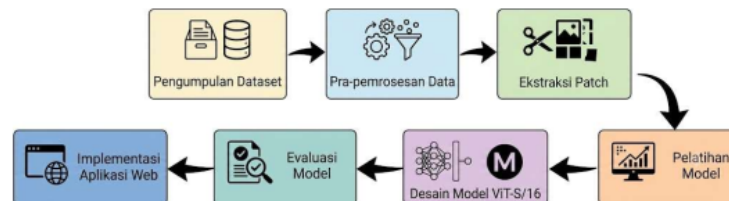
Gambar 1. Alur Penelitian
