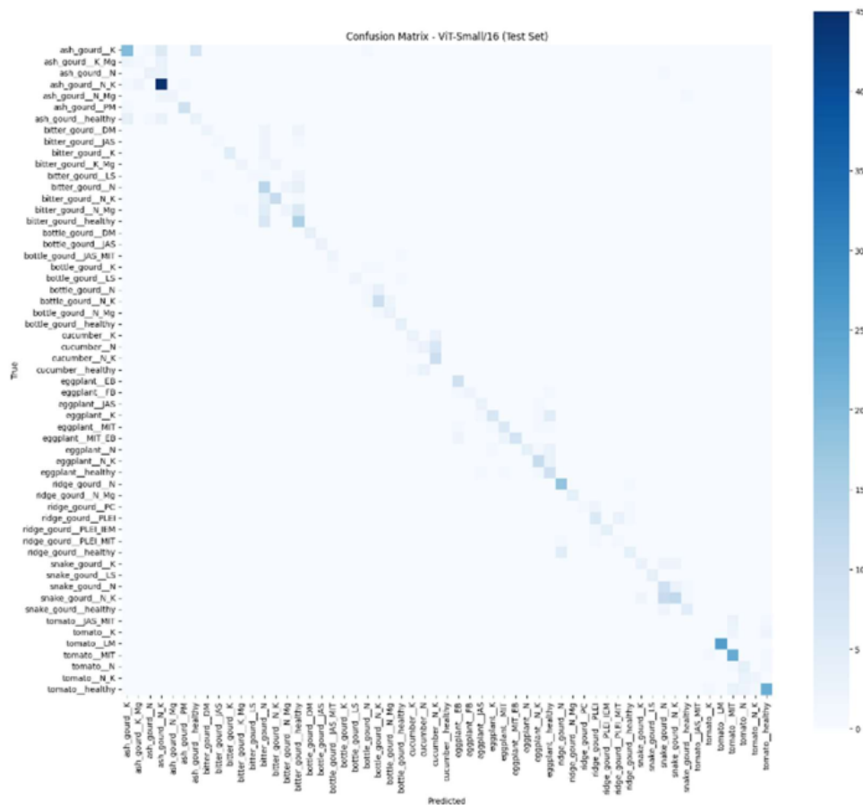
Gambar 6. Confusion Matrix
