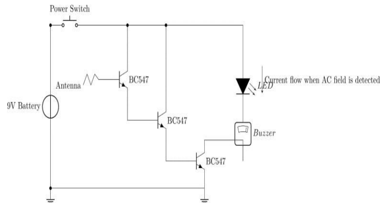
Gambar 8. Single diagram early warning system
