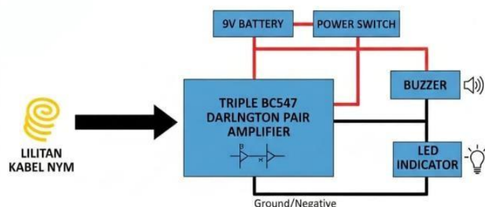
Gambar 7. Blok Diagram Early Warning System
