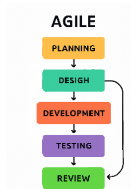
Gambar 2. Metode Agile
