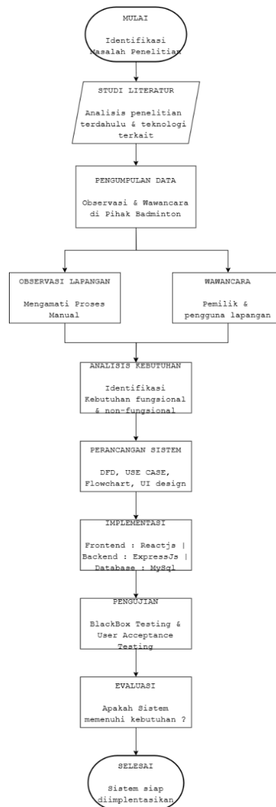
Gambar 3. Flowchart Penelitian
