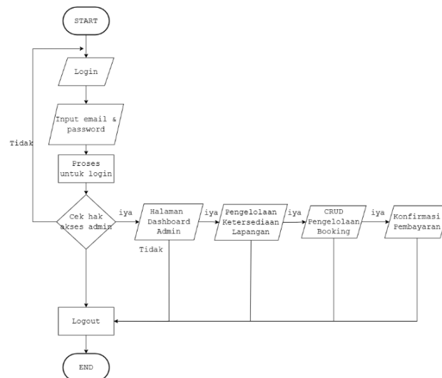
Gambar 4. Flowchart Admin
