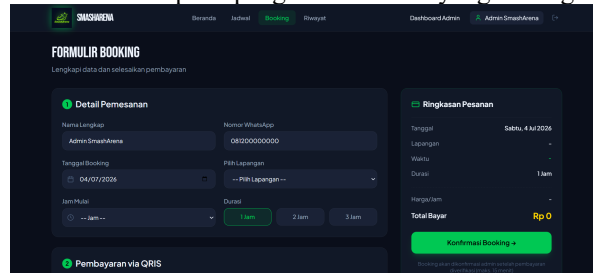
Gambar 10. Halaman Booking
