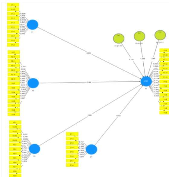
Gambar 1. Skema Outer Model
