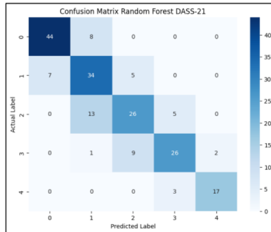
Gambar 3. Confusion Matrix Random Forest
