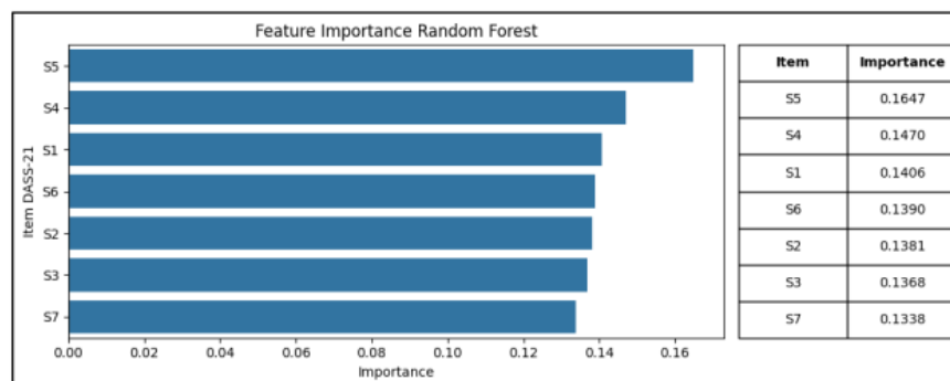
Gambar 4. Feature Importance Random Forest
