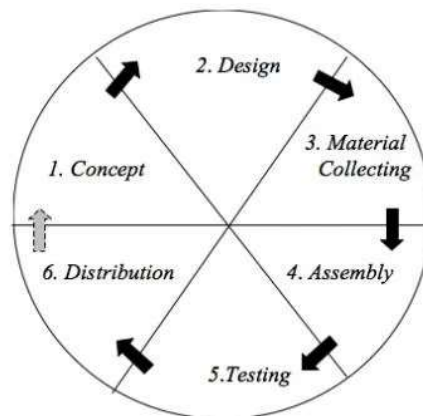
Gambar 1. Diagram MDLC (Sumber: [15])
