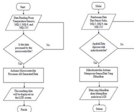
Gambar 3. Flowchart
