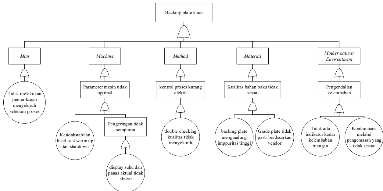
Gambar 2. Fault tree analysis backing plate karat
