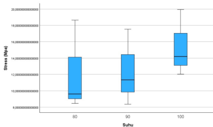
Gambar 11 Boxplot Nilai Stress terhadap Variasi Suhu
