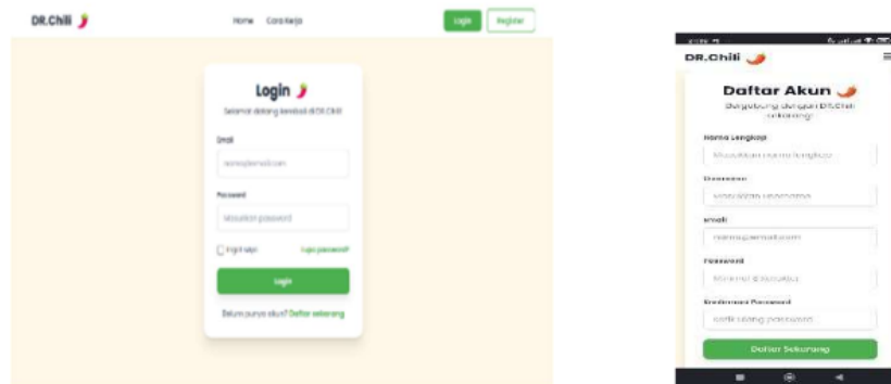
Gambar 8 Halaman Regsitration
