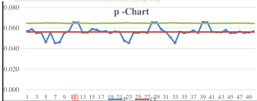
Gambar 3 Diagram Peta Kendali (P-Chart)
