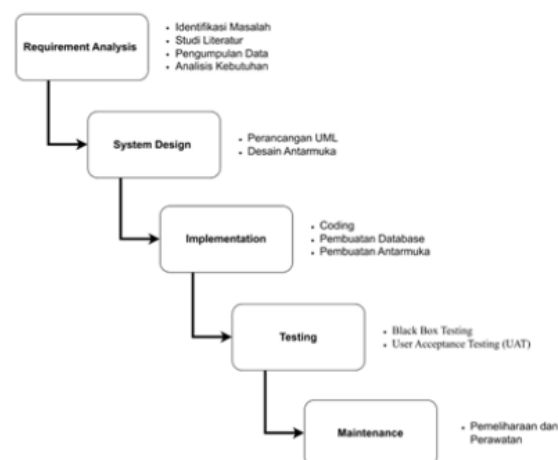
Gambar 2. Metode waterfall
