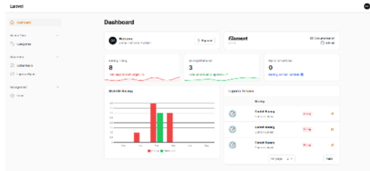
Gambar 12. Dashboard administrator
