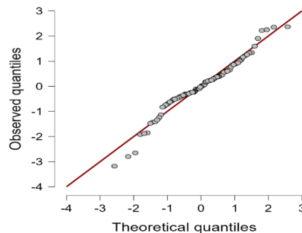
Gambar 4. Q-Q Plot Residual Terstandarisasi
