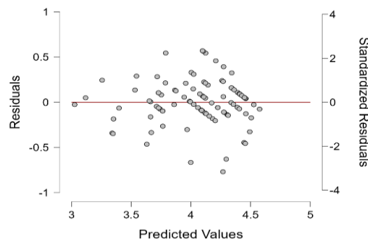
Gambar 5. Grafik Scatterplot Residuals vs Predicted
