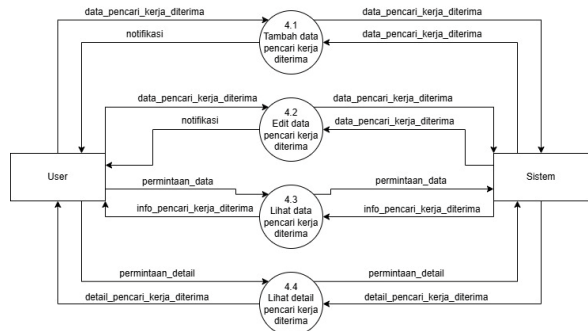
Gambar 6. DFD level 2
