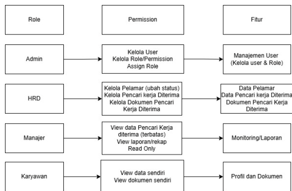
Gambar 8. Diagram RBAC
