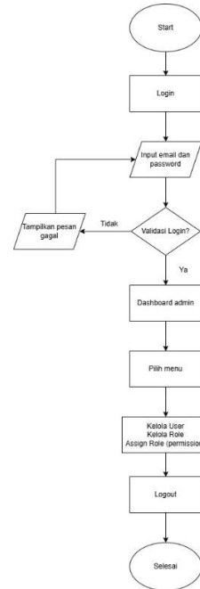
Gambar 2. Flowchart admin
