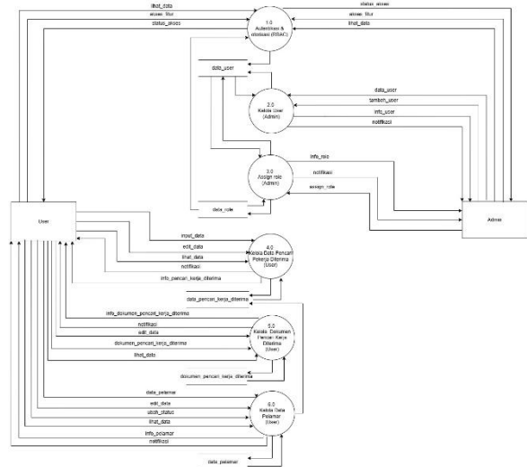
Gambar 5. DFD level 1
