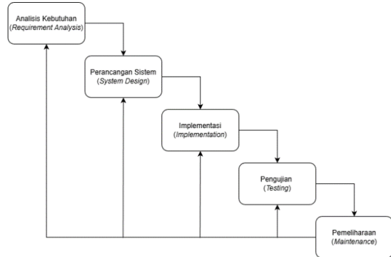
Gambar 1. Diagram waterfall
