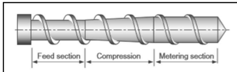
Gambar 2. Bagian zona single screw
