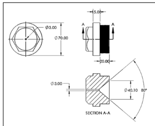
Gambar 8. Geometri dies
