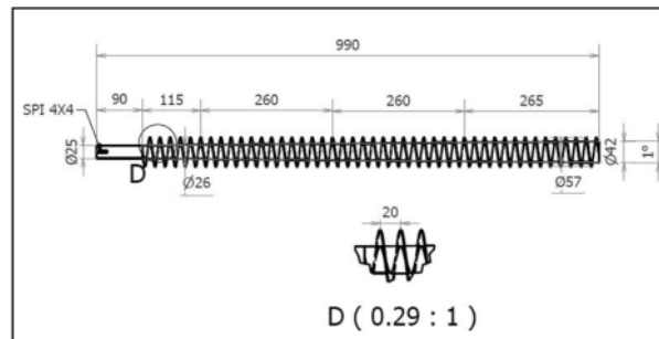
Gambar 3. Desain 2 Dimensi Single crew
