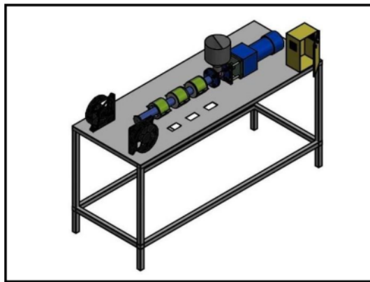
Gambar 1. Desain Mesin Extruder single screw
