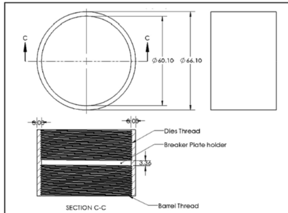
Gambar 9. Geometri Dies Housing
