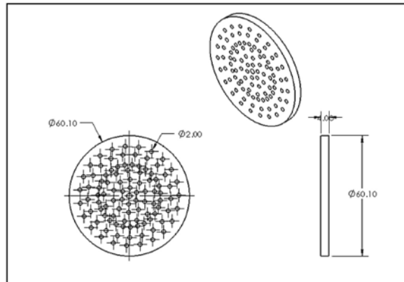
Gambar 7. Geometri Breaker Plate
