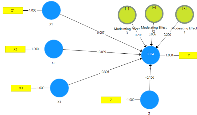
Gambar 1. Outer Model Atau Measurement Model
