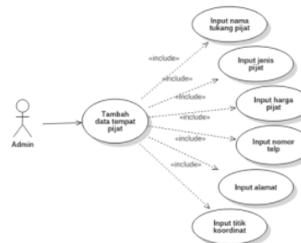
Gambar 4. Use Case Diagram tambah data
