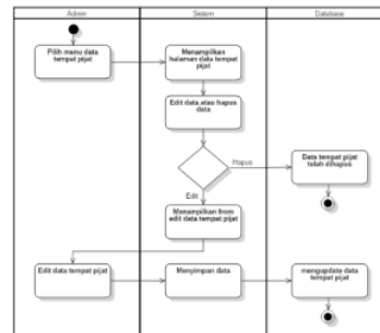
Gambar 8. Diagram Activity kelola data
