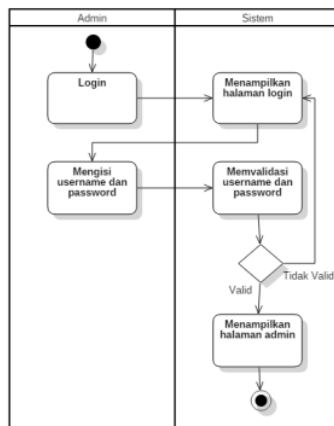
Gambar 7. Diagram Activity login admin
