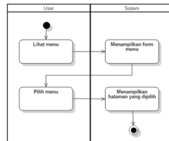
Gambar 10. Diagram Activity user
