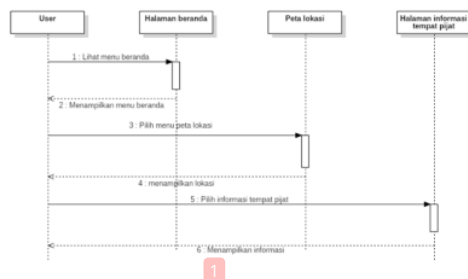
Gambar 12. Sequence diagram user
