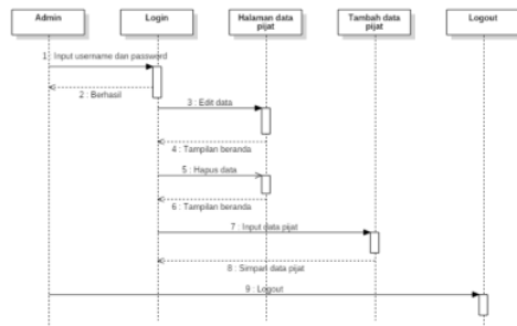
Gambar 11. Sequence diagram admin
