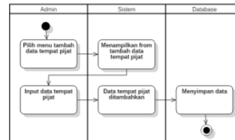
Gambar 9. Diagram Activity tambah data
